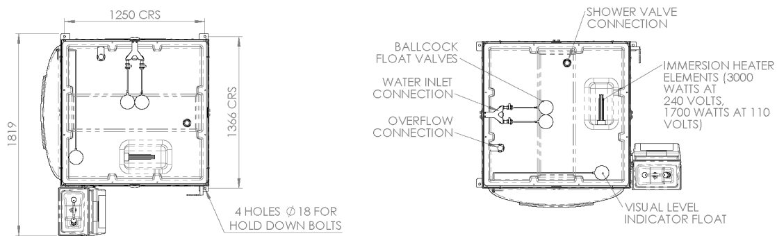
PLAN VIEWS WITH ROOF OMITTED
